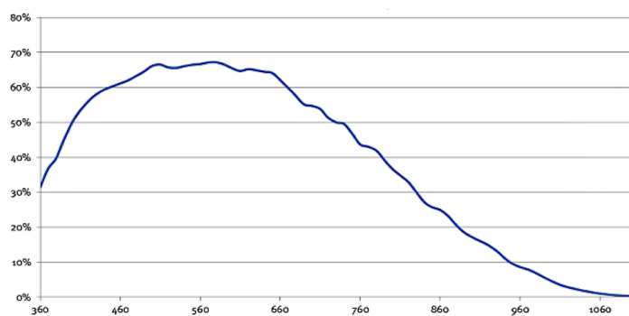
Quantum Efficiency Curve for Mono Sensor
