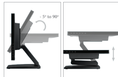
Flexible dual-hinge stand design to maximise viewing comfort for multiple users
