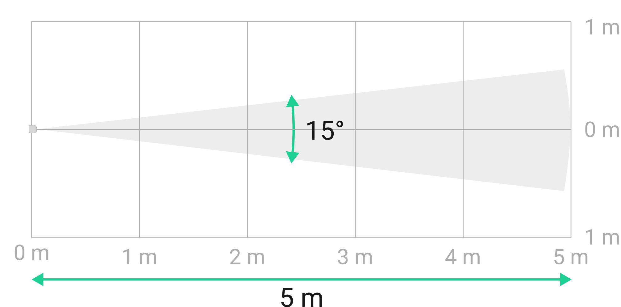
Installation oben
