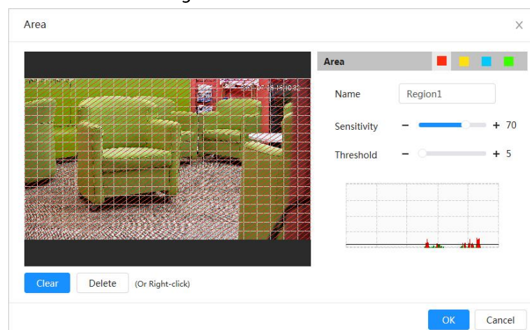
Figure 4-71 Area
