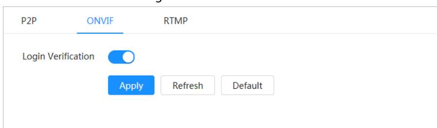
Figure 4-43 ONVIF
