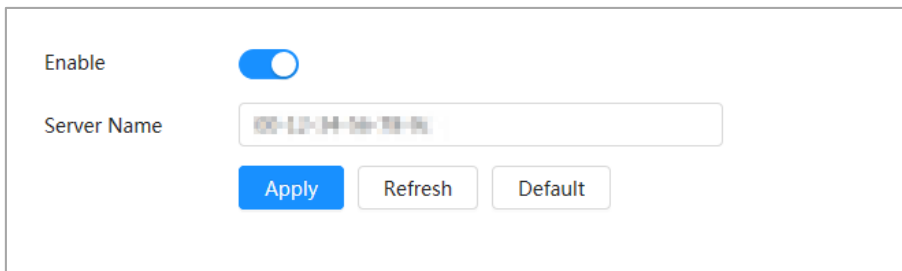
Figure 4-38 Bonjour
