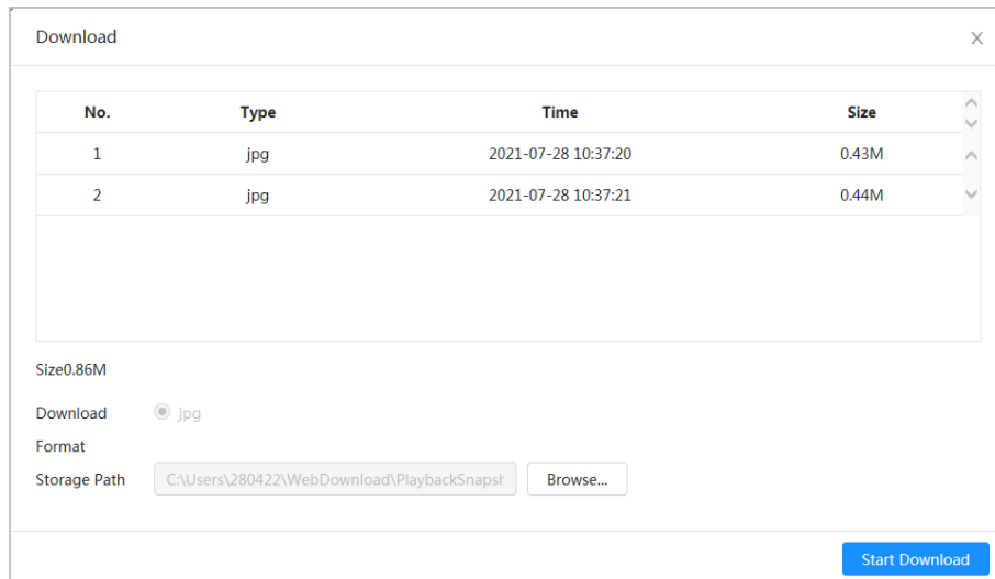
Figure 7-4 Downloading image
