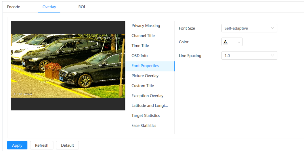
Figure 4-20 Font properties
