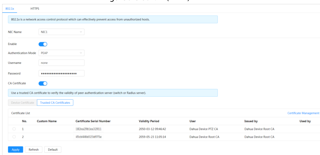
Figure 9-3 802.1x (PEAP)
