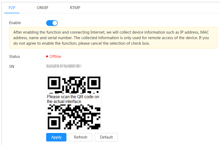
Figure 4-42 P2P
