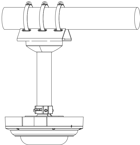
Pole Mount(Horizontal)
