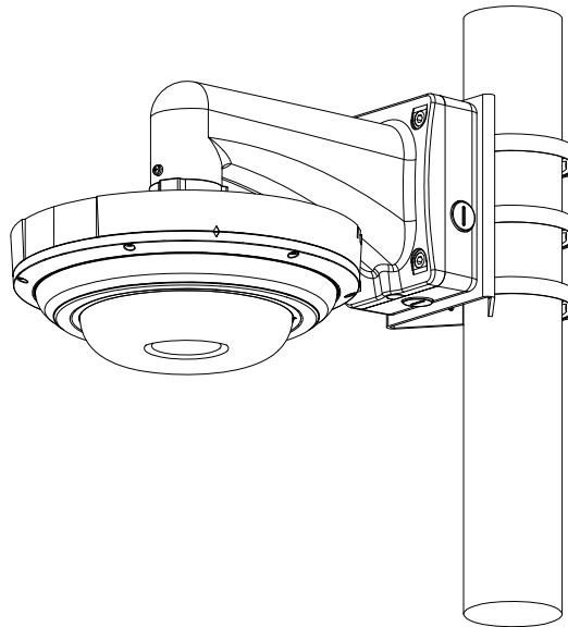
Pole Mount(Vertical)
